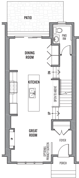
MAIN FLOOR PLAN 700 SQ.FT.
